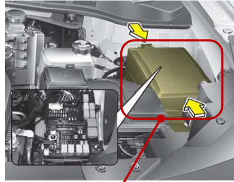
Engine room fuse box
