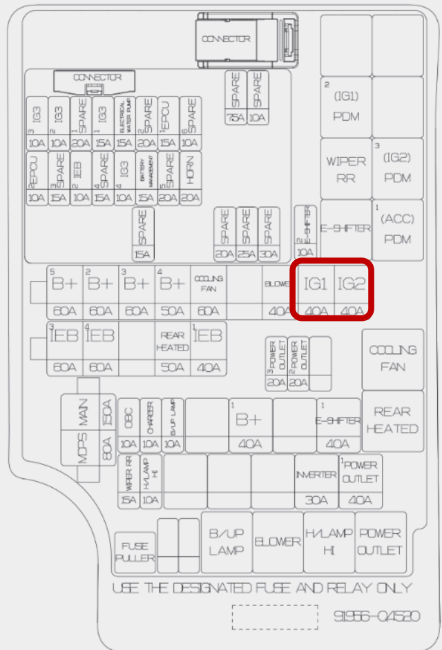
Engine room fuse box
